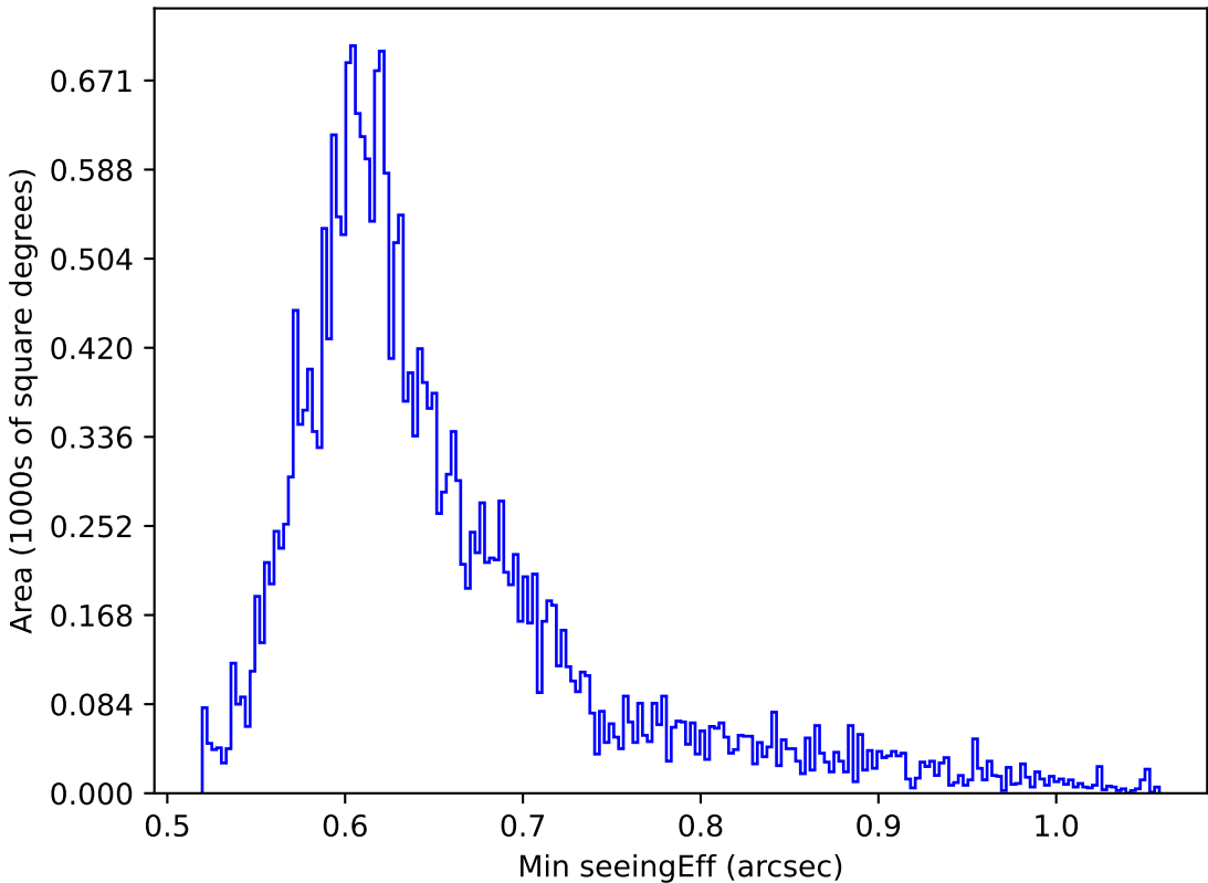
too_elab_r64_d3_giz_v3.4_10yrs All sky z band: Min seeingEff
