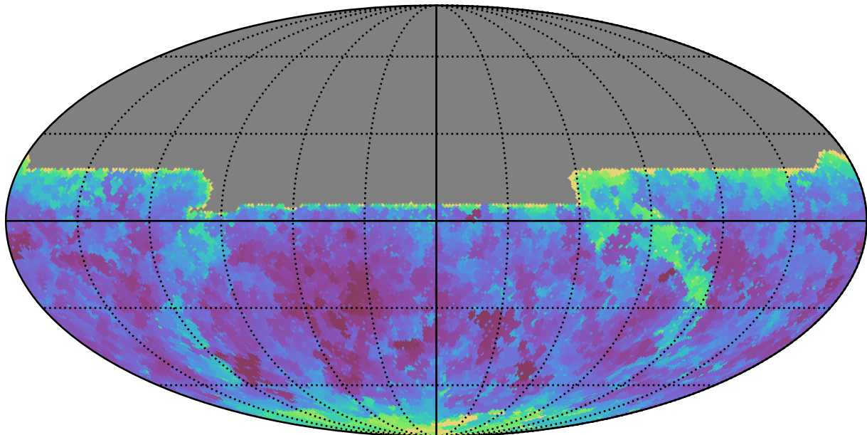
too_elab_r64_d3_giz_v3.4_10yrs All sky y band: Min seeingEff
