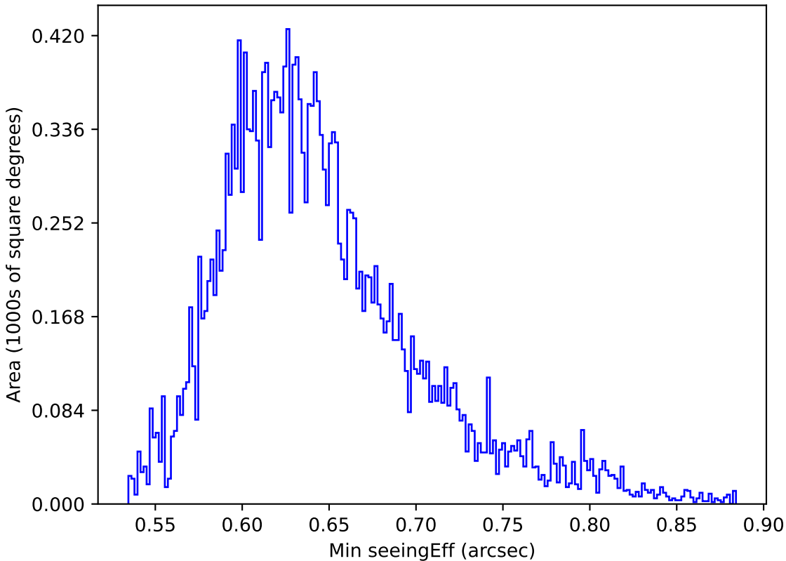
too_elab_r64_d3_giz_v3.4_10yrs All sky y band: Min seeingEff
