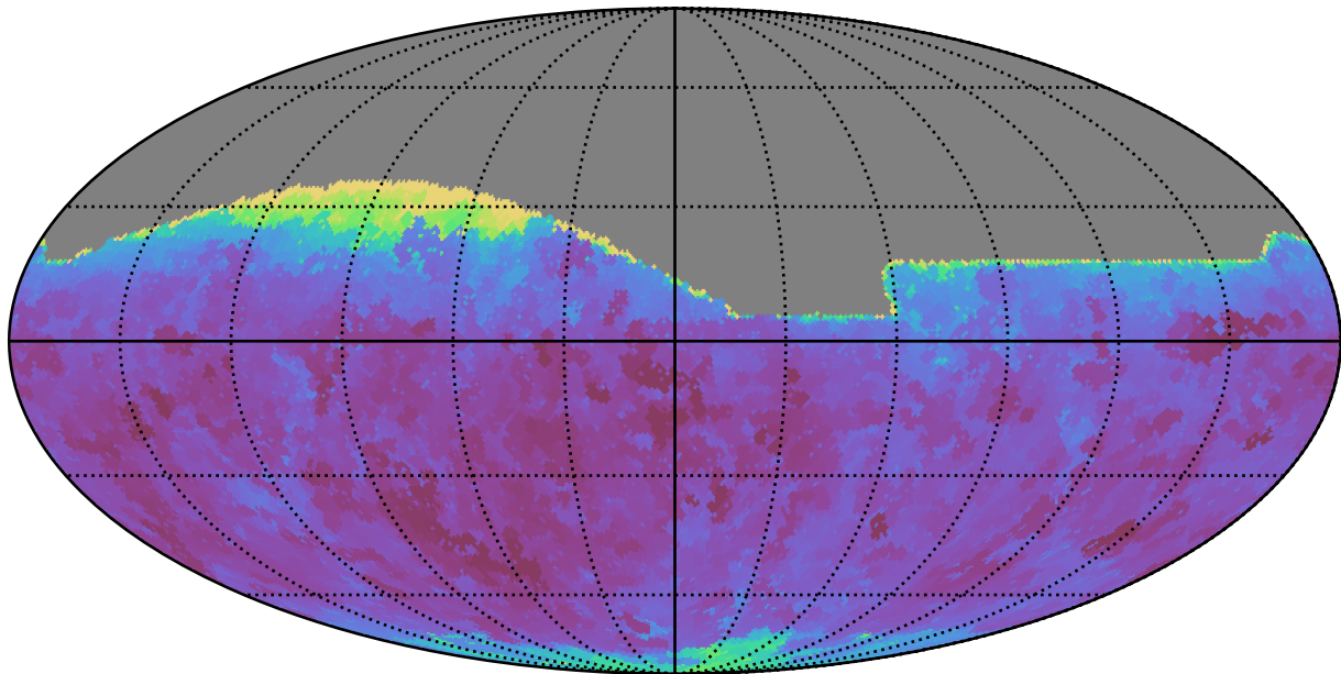
too_elab_r64_d3_giz_v3.4_10yrs All sky r band: Min seeingEff
