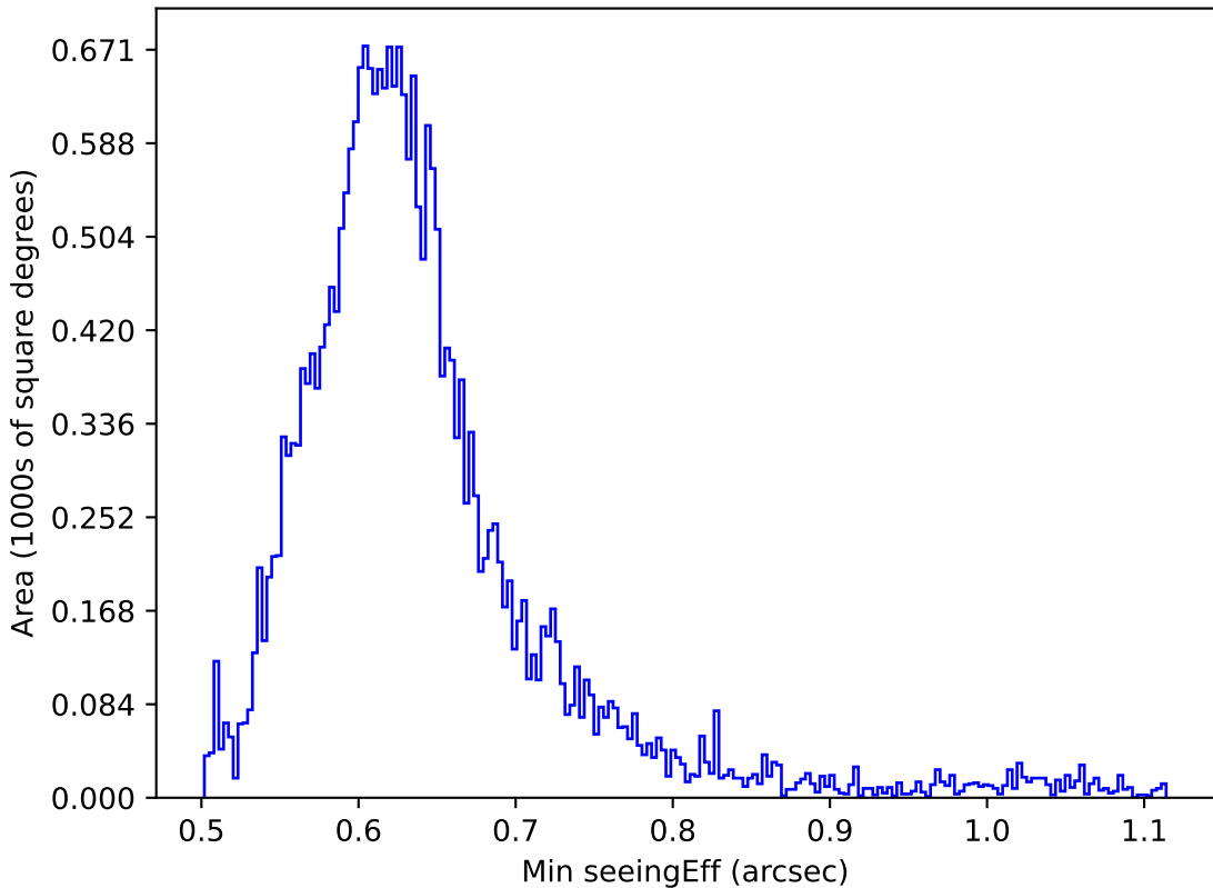
too_elab_r64_d3_giz_v3.4_10yrs All sky r band: Min seeingEff
