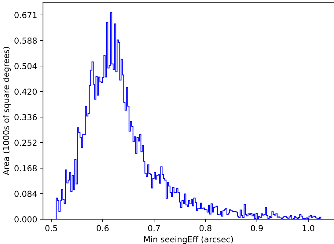
too_elab_r64_d3_giz_v3.4_10yrs All sky i band: Min seeingEff
