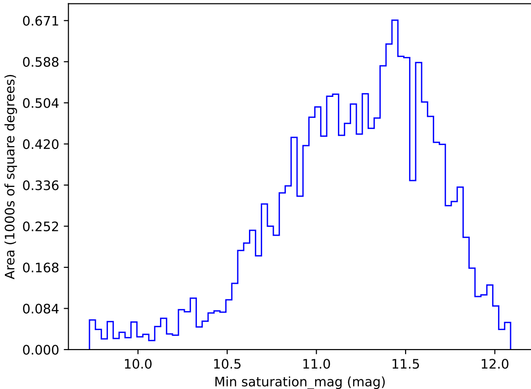
too_elab_r64_d3_giz_v3.4_10yrs WFD y band: Min saturation_mag
