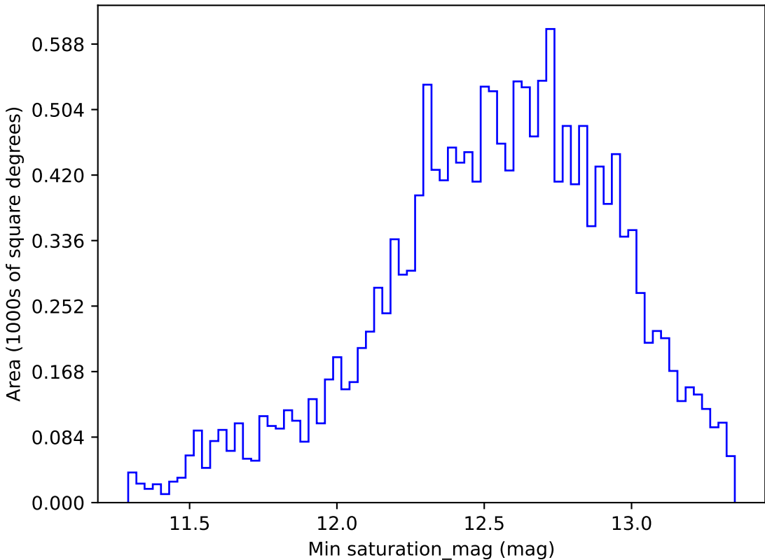
too_elab_r64_d3_giz_v3.4_10yrs WFD r band: Min saturation_mag
