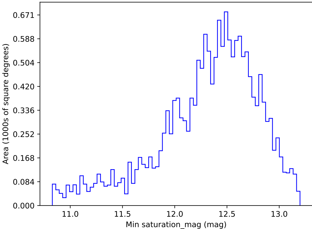
too_elab_r64_d3_giz_v3.4_10yrs WFD i band: Min saturation_mag
