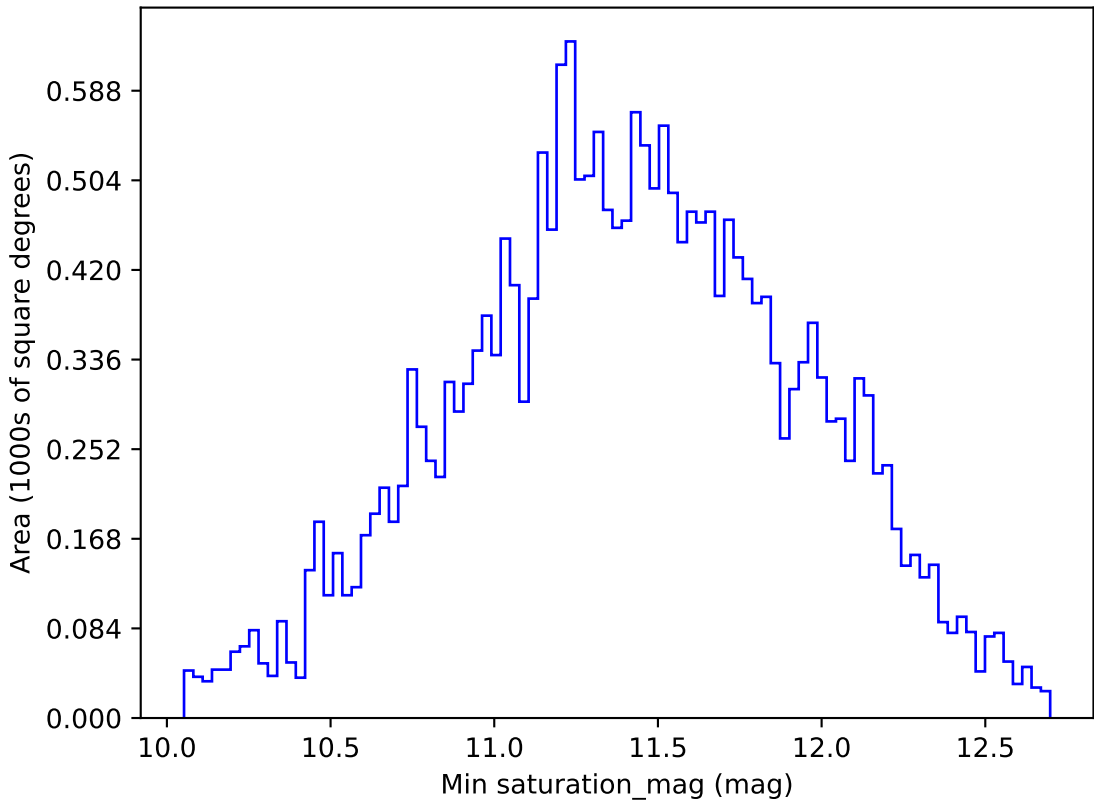
too_elab_r64_d3_giz_v3.4_10yrs All sky u band: Min saturation_mag
