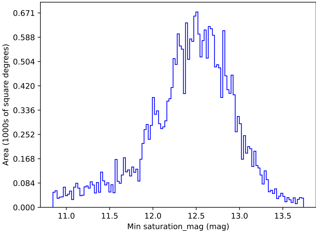
too_elab_r64_d3_giz_v3.4_10yrs All sky i band: Min saturation_mag
