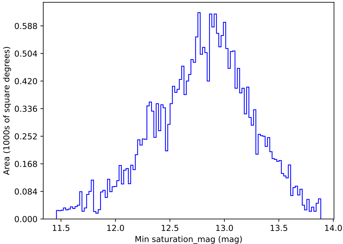
too_elab_r64_d3_giz_v3.4_10yrs All sky g band: Min saturation_mag
