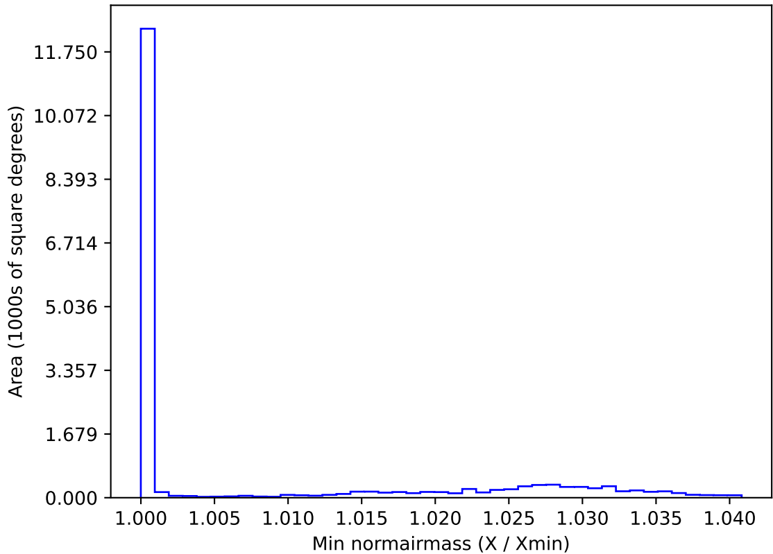
too_elab_r64_d3_giz_v3.4_10yrs WFD y band: Min normairmass
