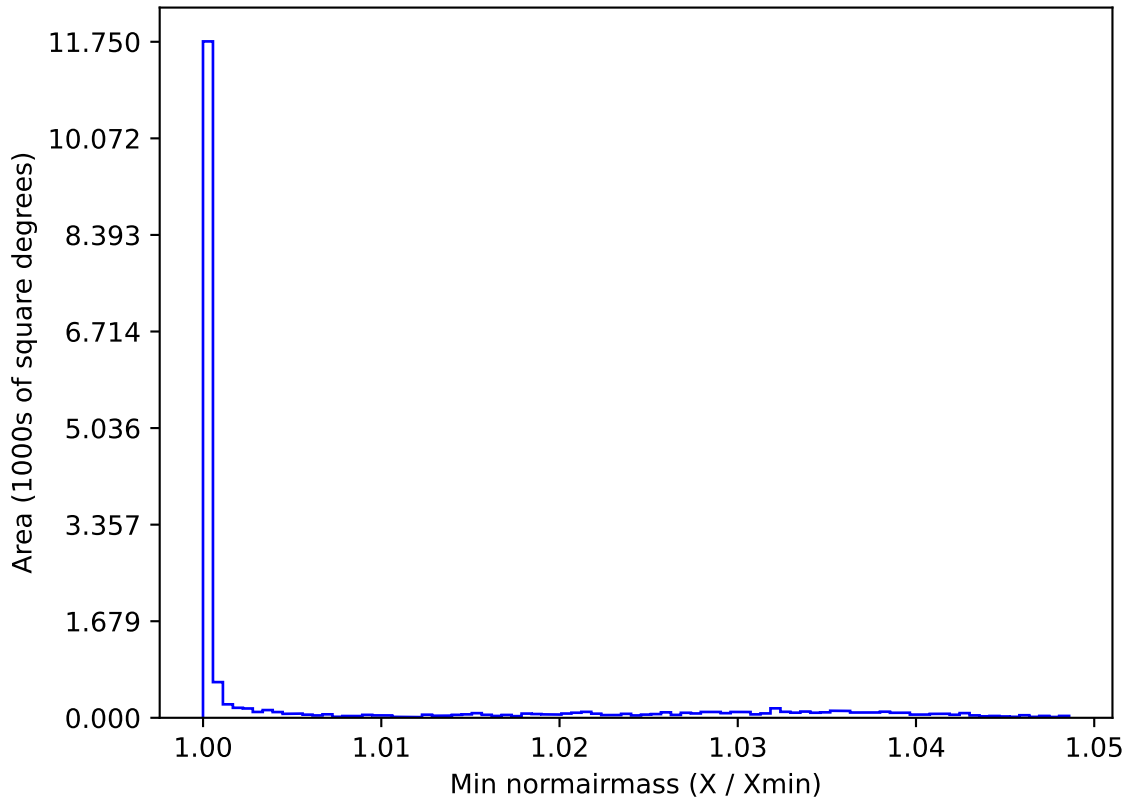
too_elab_r64_d3_giz_v3.4_10yrs WFD g band: Min normairmass
