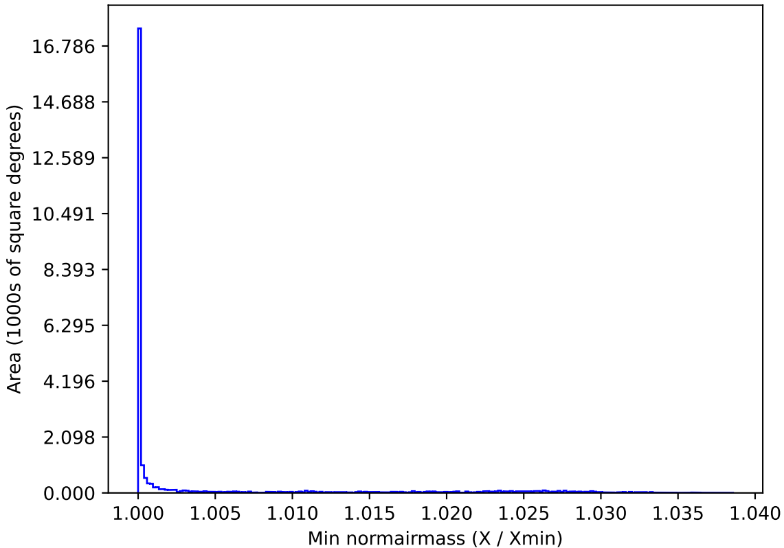
too_elab_r64_d3_giz_v3.4_10yrs All sky z band: Min normairmass
