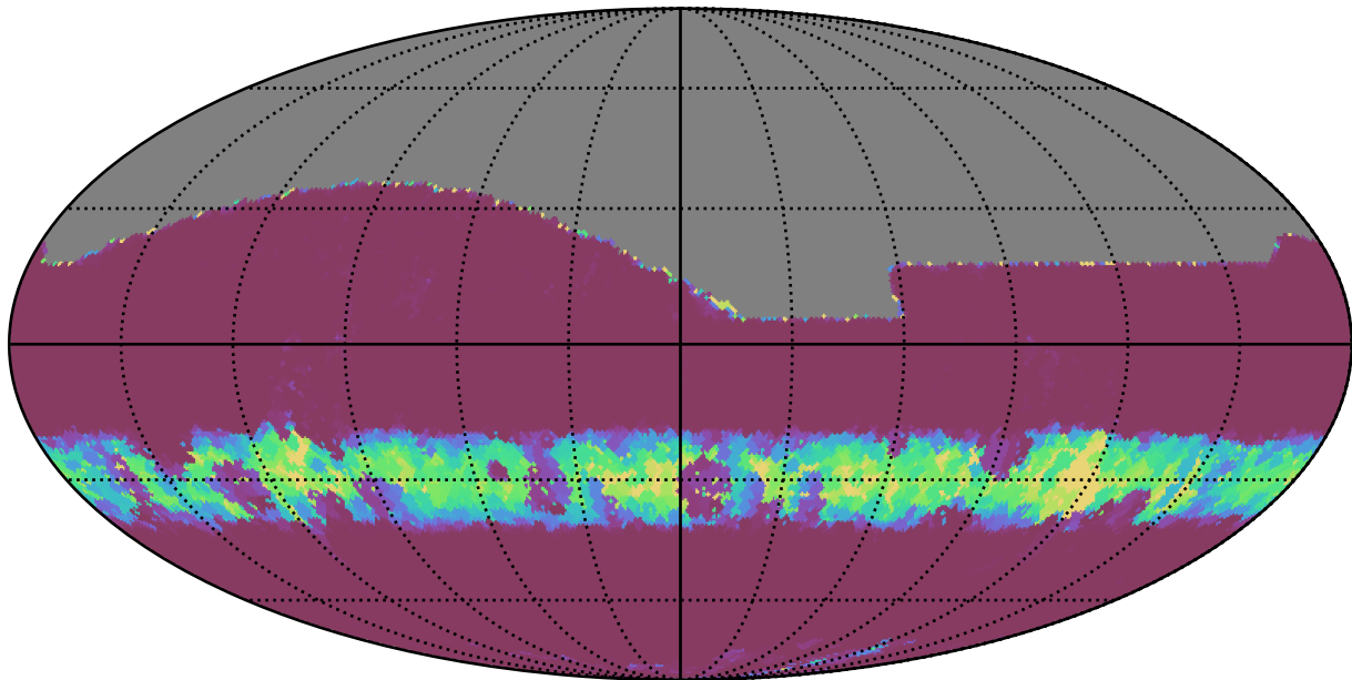
too_elab_r64_d3_giz_v3.4_10yrs All sky i band: Min normairmass
