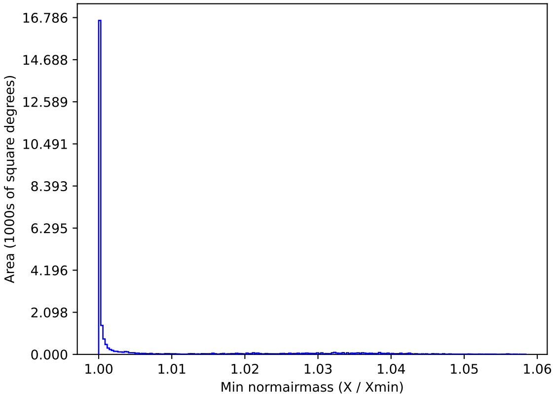
too_elab_r64_d3_giz_v3.4_10yrs All sky g band: Min normairmass
