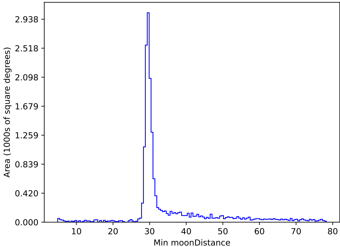
too_elab_r64_d3_giz_v3.4_10yrs WFD z band: Min moonDistance
