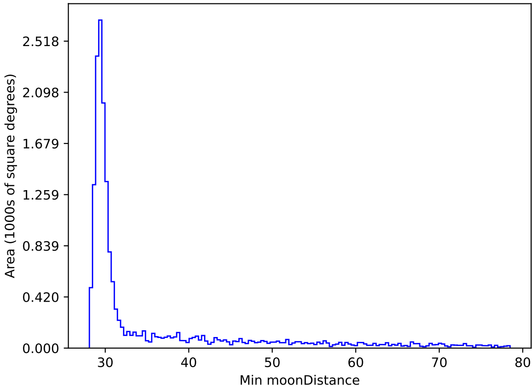
too_elab_r64_d3_giz_v3.4_10yrs WFD y band: Min moonDistance
