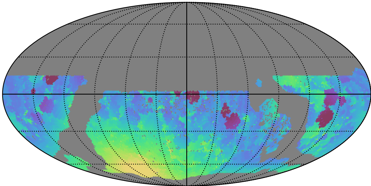
too_elab_r64_d3_giz_v3.4_10yrs WFD g band: Min moonDistance
