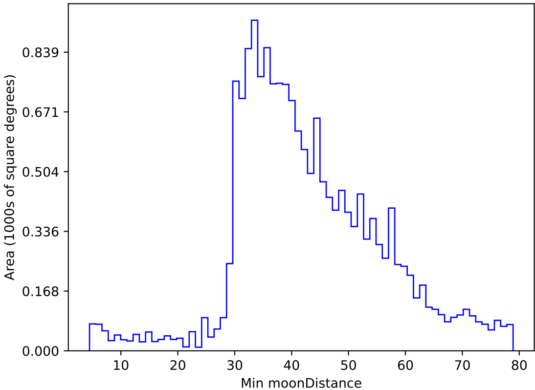
too_elab_r64_d3_giz_v3.4_10yrs WFD g band: Min moonDistance
