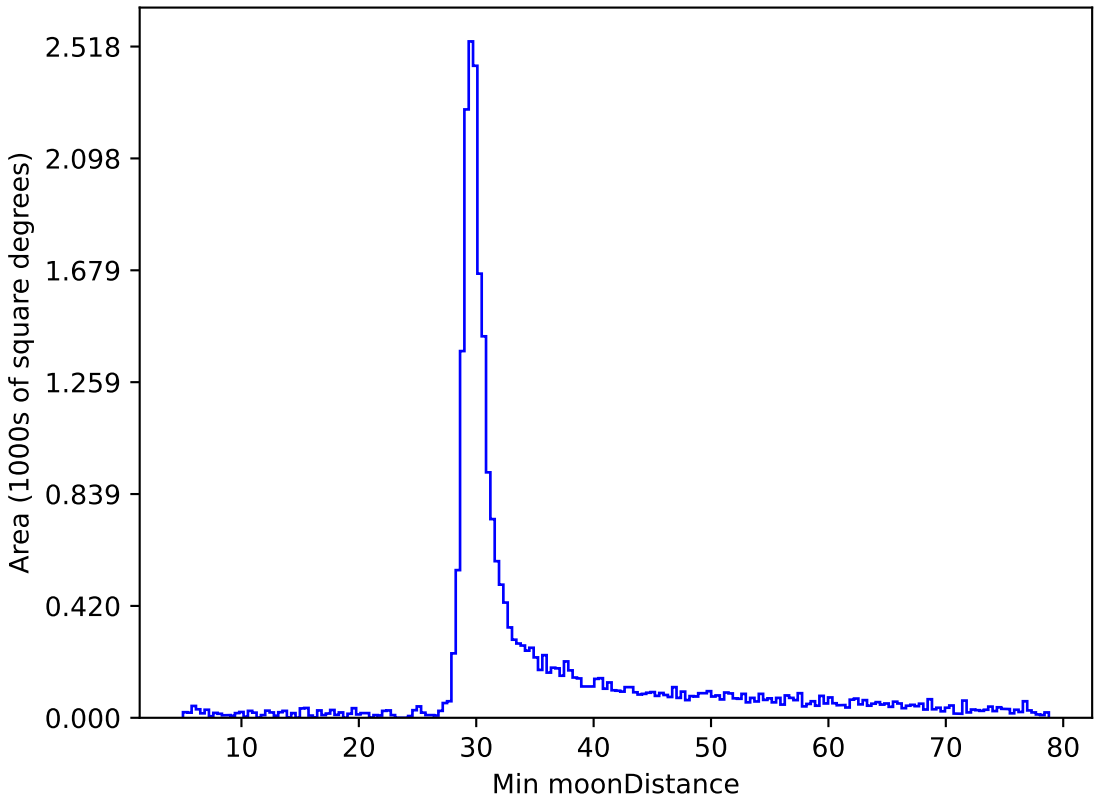
too_elab_r64_d3_giz_v3.4_10yrs All sky z band: Min moonDistance
