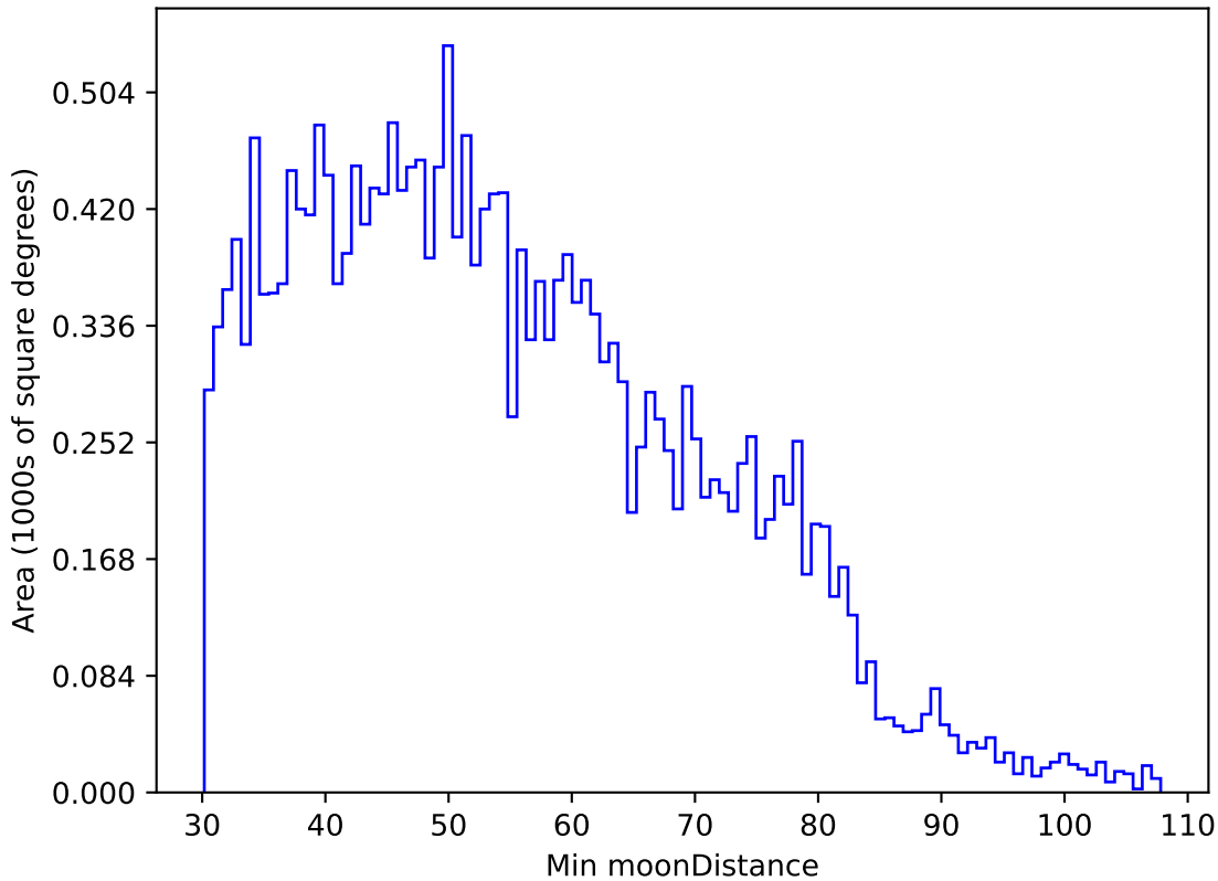
too_elab_r64_d3_giz_v3.4_10yrs All sky u band: Min moonDistance
