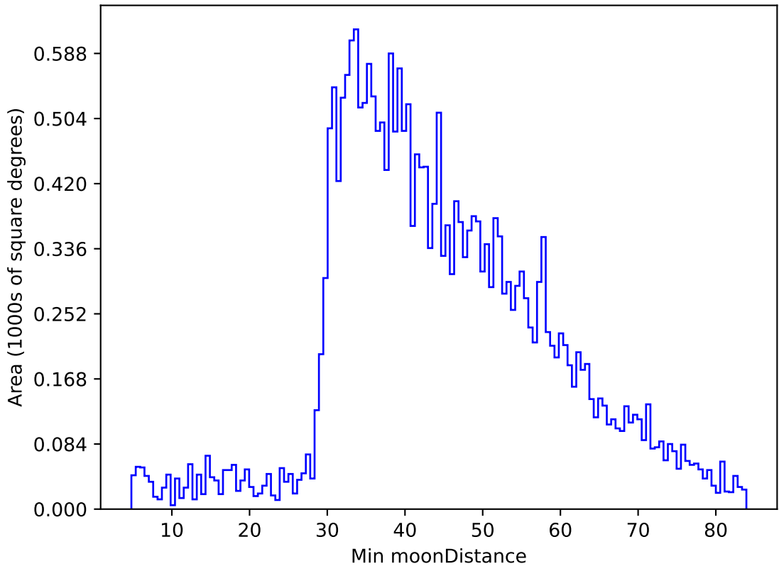
too_elab_r64_d3_giz_v3.4_10yrs All sky g band: Min moonDistance
