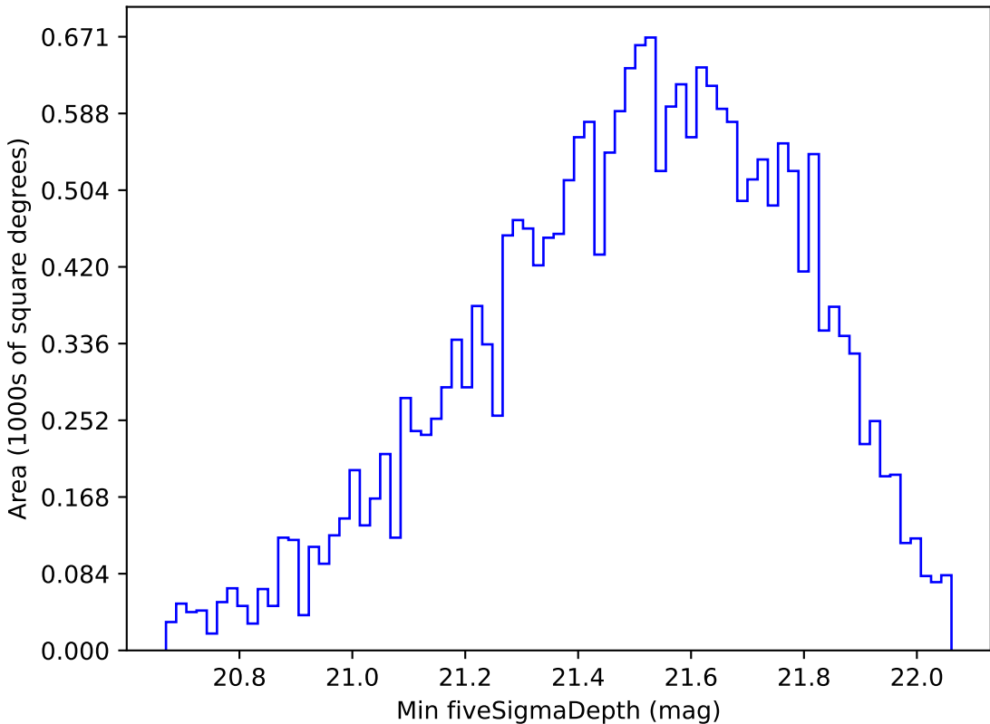
too_elab_r64_d3_giz_v3.4_10yrs Yr 1 y band: Min fiveSigmaDepth
