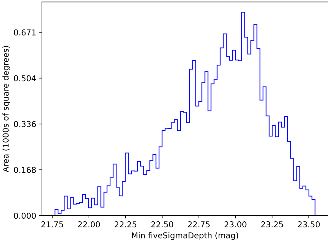
too_elab_r64_d3_giz_v3.4_10yrs Yr 1 u band: Min fiveSigmaDepth
