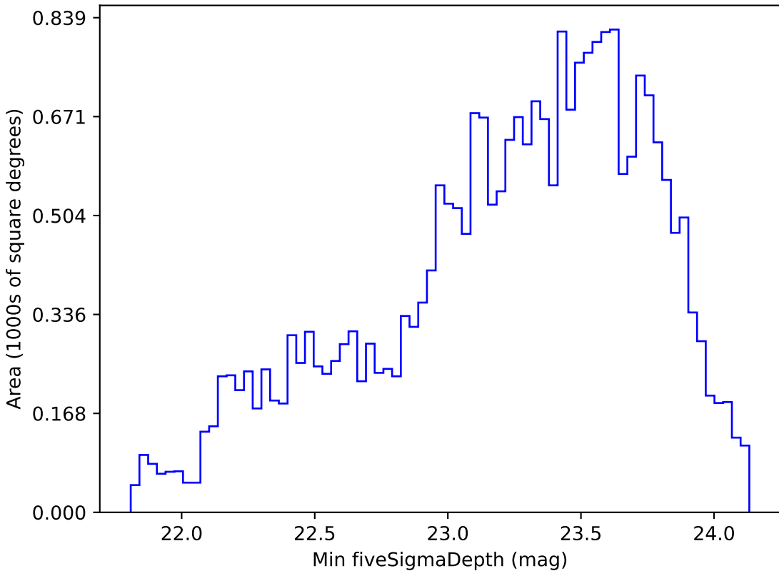
too_elab_r64_d3_giz_v3.4_10yrs Yr 1 r band: Min fiveSigmaDepth
