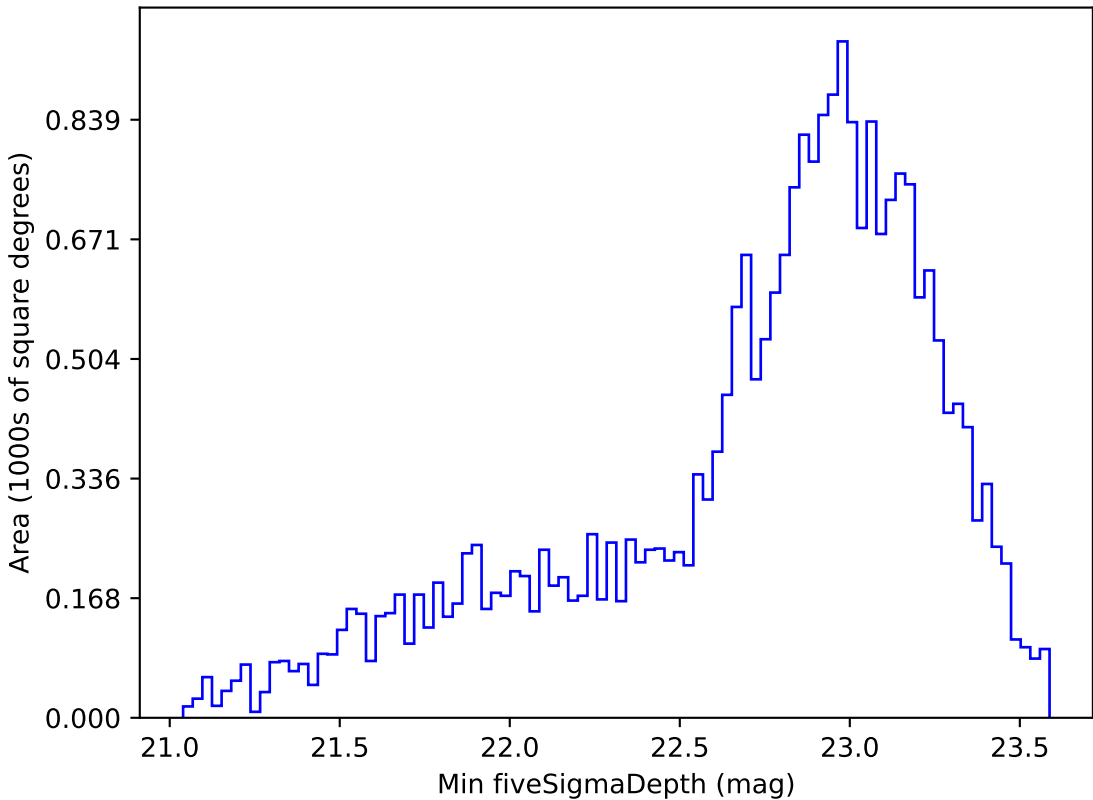
too_elab_r64_d3_giz_v3.4_10yrs Yr 1 i band: Min fiveSigmaDepth
