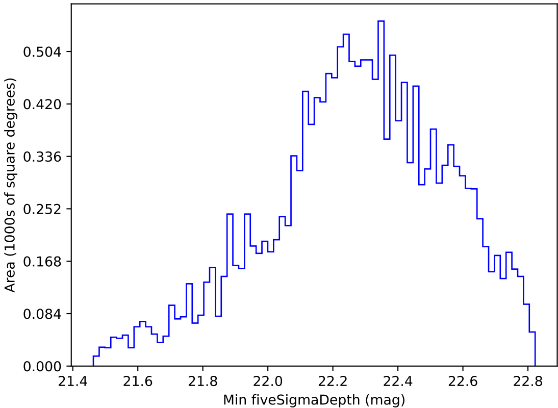
too_elab_r64_d3_giz_v3.4_10yrs WFD u band: Min fiveSigmaDepth
