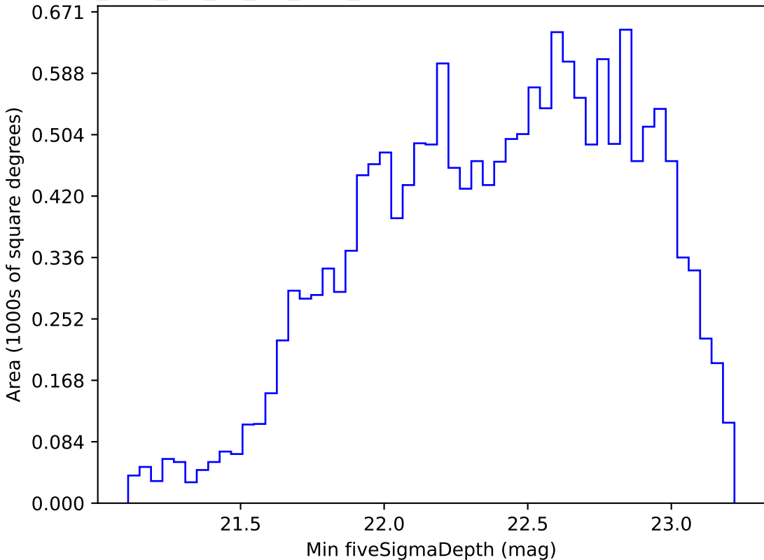
too_elab_r64_d3_giz_v3.4_10yrs WFD r band: Min fiveSigmaDepth
