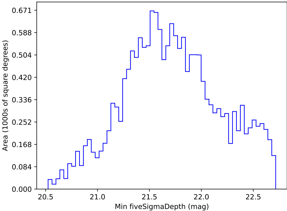
too_elab_r64_d3_giz_v3.4_10yrs WFD i band: Min fiveSigmaDepth
