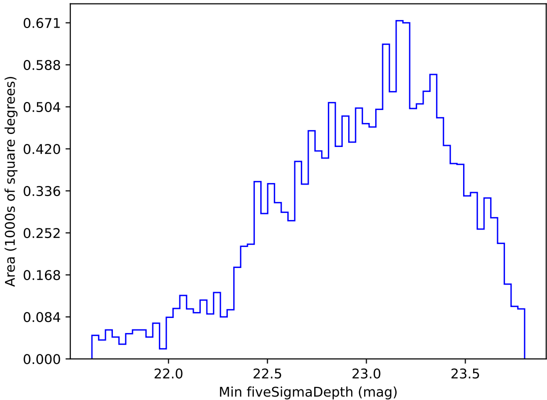
too_elab_r64_d3_giz_v3.4_10yrs WFD g band: Min fiveSigmaDepth
