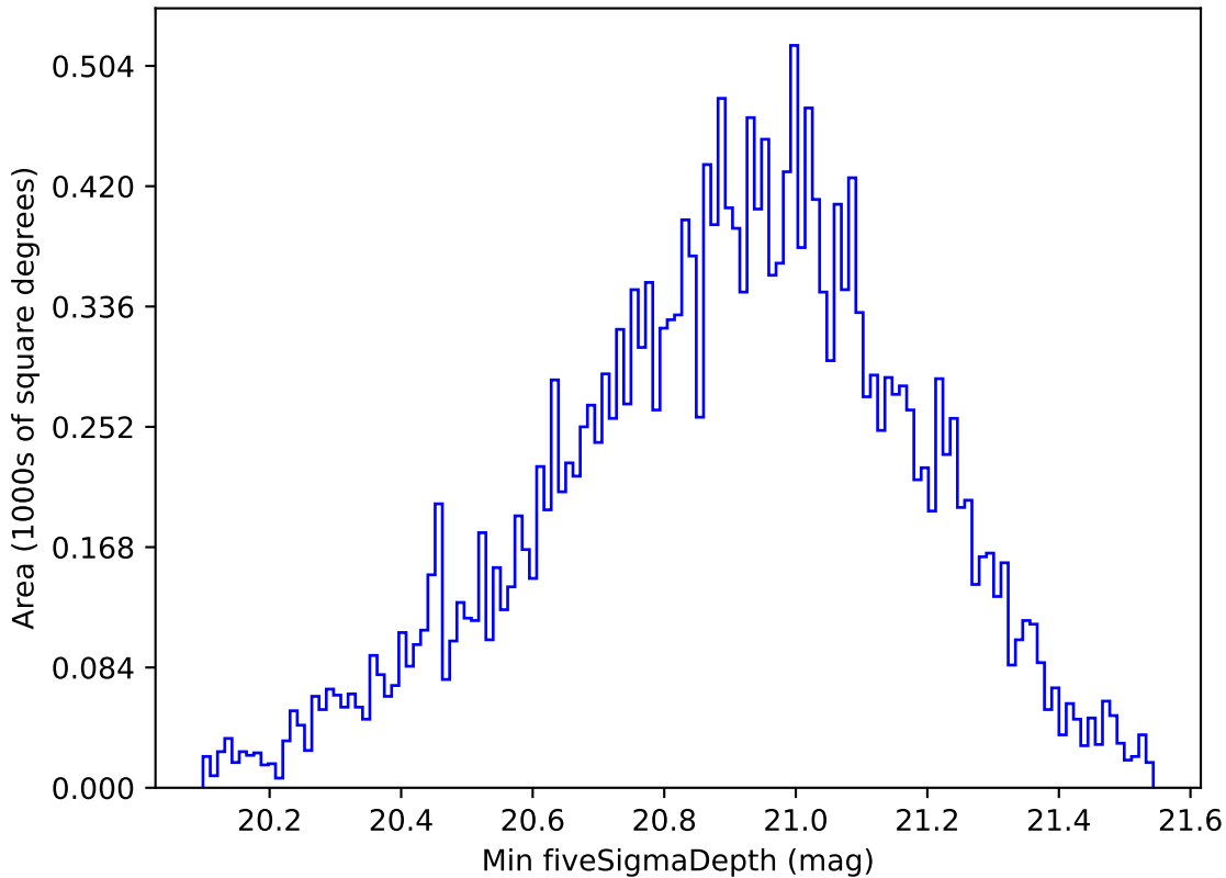
too_elab_r64_d3_giz_v3.4_10yrs All sky y band: Min fiveSigmaDepth
