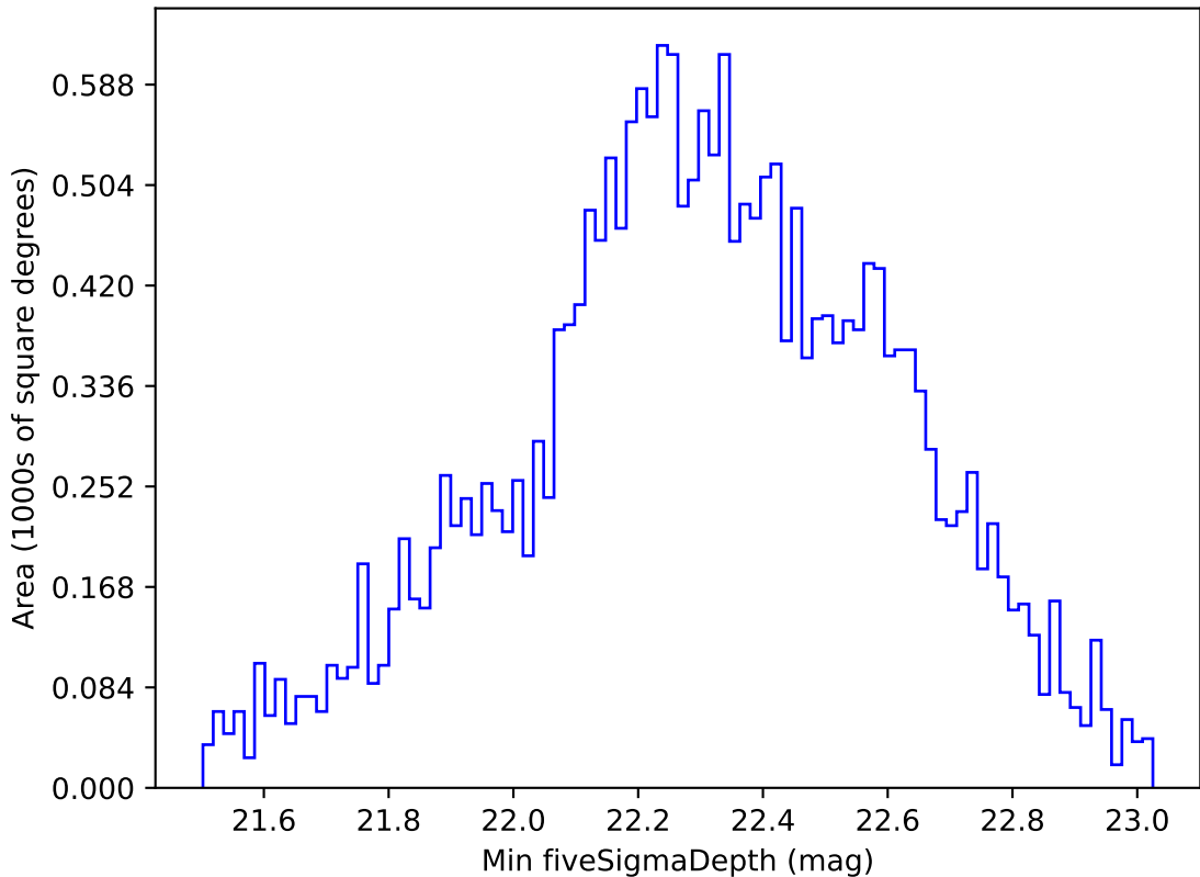
too_elab_r64_d3_giz_v3.4_10yrs All sky u band: Min fiveSigmaDepth
