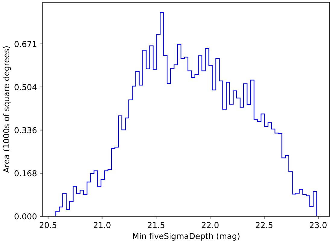
too_elab_r64_d3_giz_v3.4_10yrs All sky i band: Min fiveSigmaDepth
