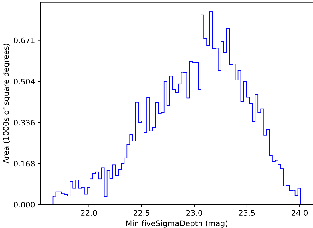
too_elab_r64_d3_giz_v3.4_10yrs All sky g band: Min fiveSigmaDepth
