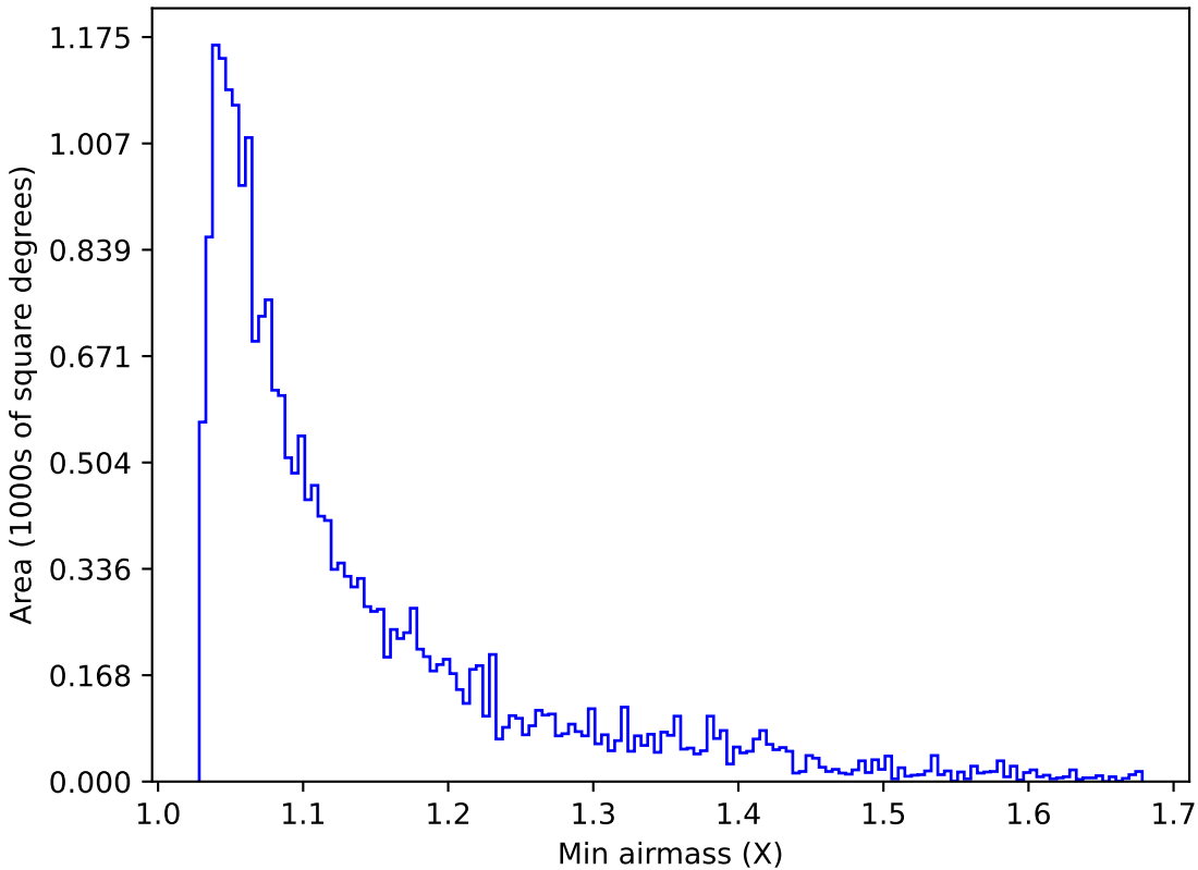
too_elab_r64_d3_giz_v3.4_10yrs Yr 1 u band: Min airmass
