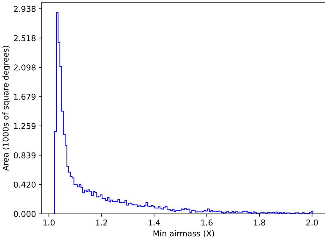
too_elab_r64_d3_giz_v3.4_10yrs Yr 1 r band: Min airmass
