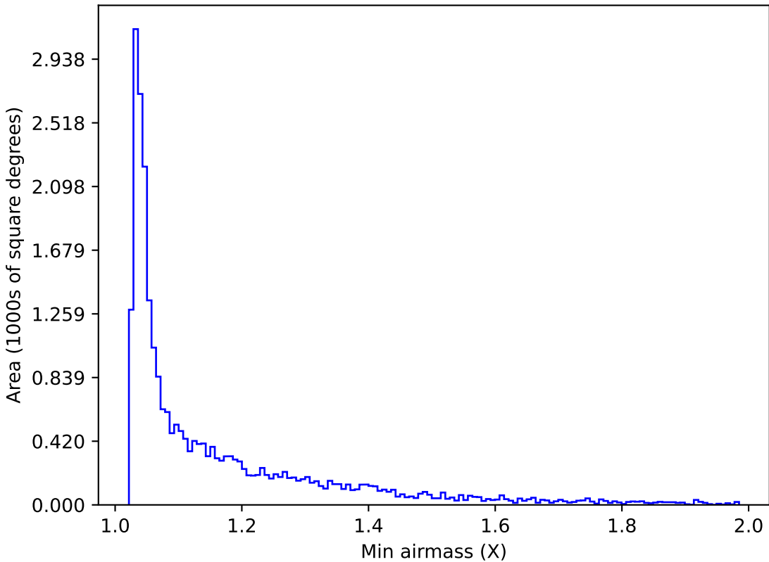
too_elab_r64_d3_giz_v3.4_10yrs Yr 1 i band: Min airmass
