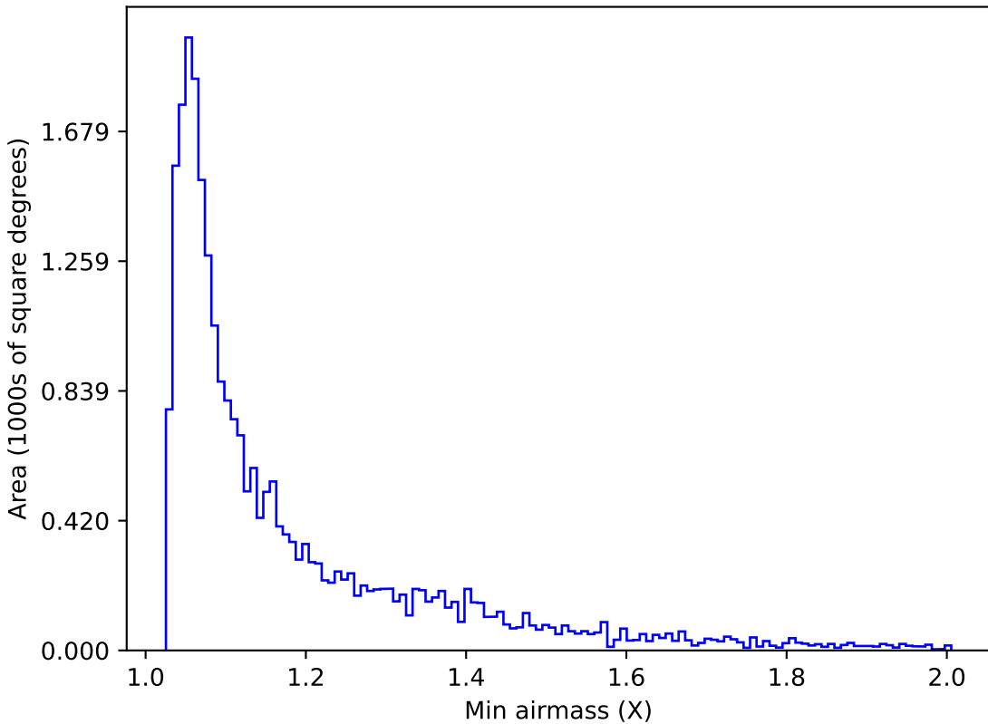
too_elab_r64_d3_giz_v3.4_10yrs Yr 1 g band: Min airmass
