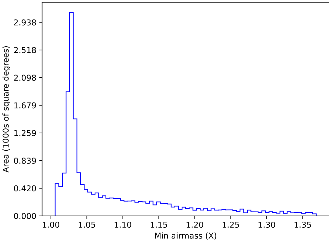
too_elab_r64_d3_giz_v3.4_10yrs WFD z band: Min airmass
