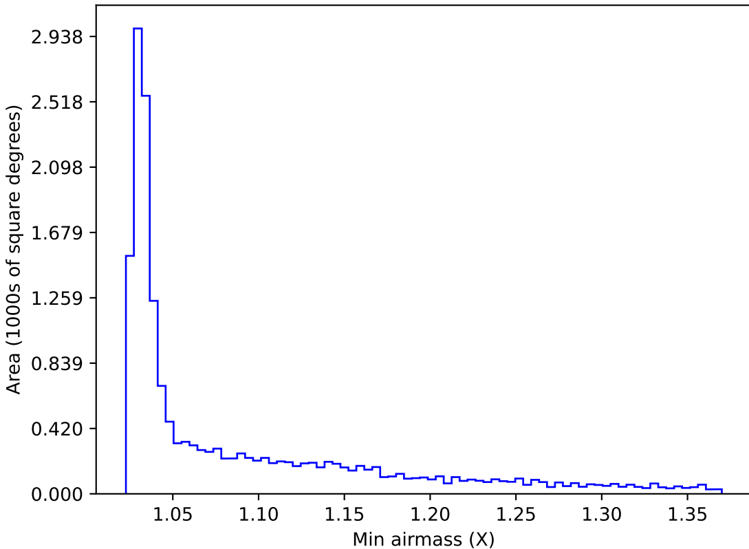
too_elab_r64_d3_giz_v3.4_10yrs WFD y band: Min airmass
