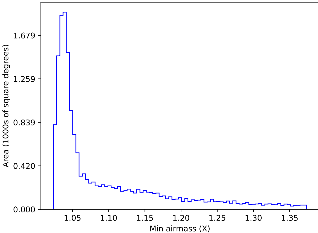
too_elab_r64_d3_giz_v3.4_10yrs WFD u band: Min airmass
