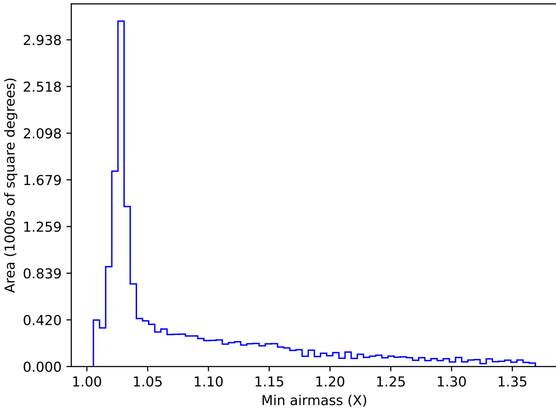
too_elab_r64_d3_giz_v3.4_10yrs WFD i band: Min airmass
