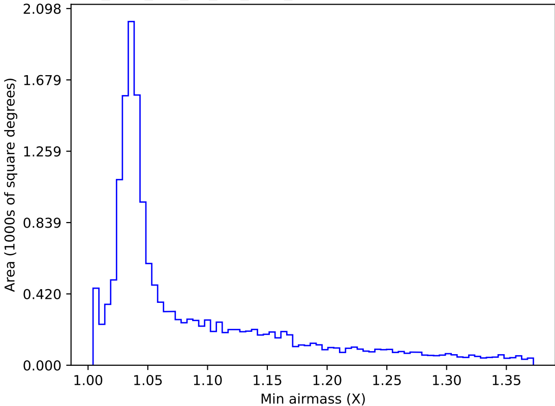
too_elab_r64_d3_giz_v3.4_10yrs WFD g band: Min airmass
