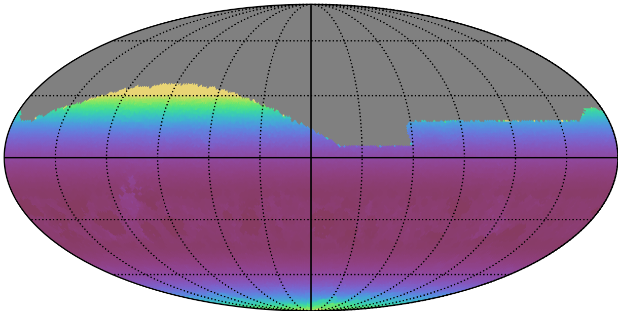
too_elab_r64_d3_giz_v3.4_10yrs All sky g band: Min airmass
