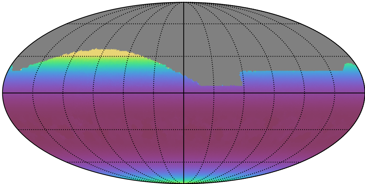
too_elab_r64_d3_giz_v3.4_10yrs All sky all bands: Min airmass
