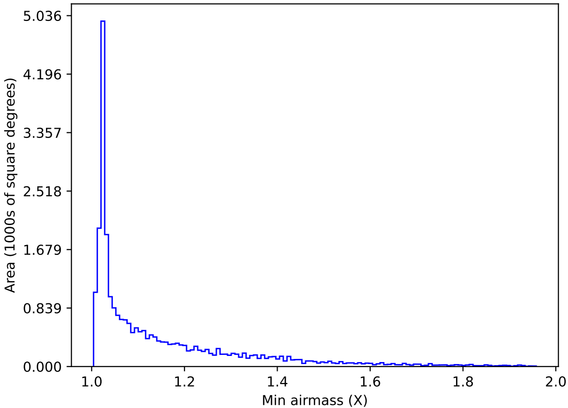
too_elab_r64_d3_giz_v3.4_10yrs All sky all bands: Min airmass
