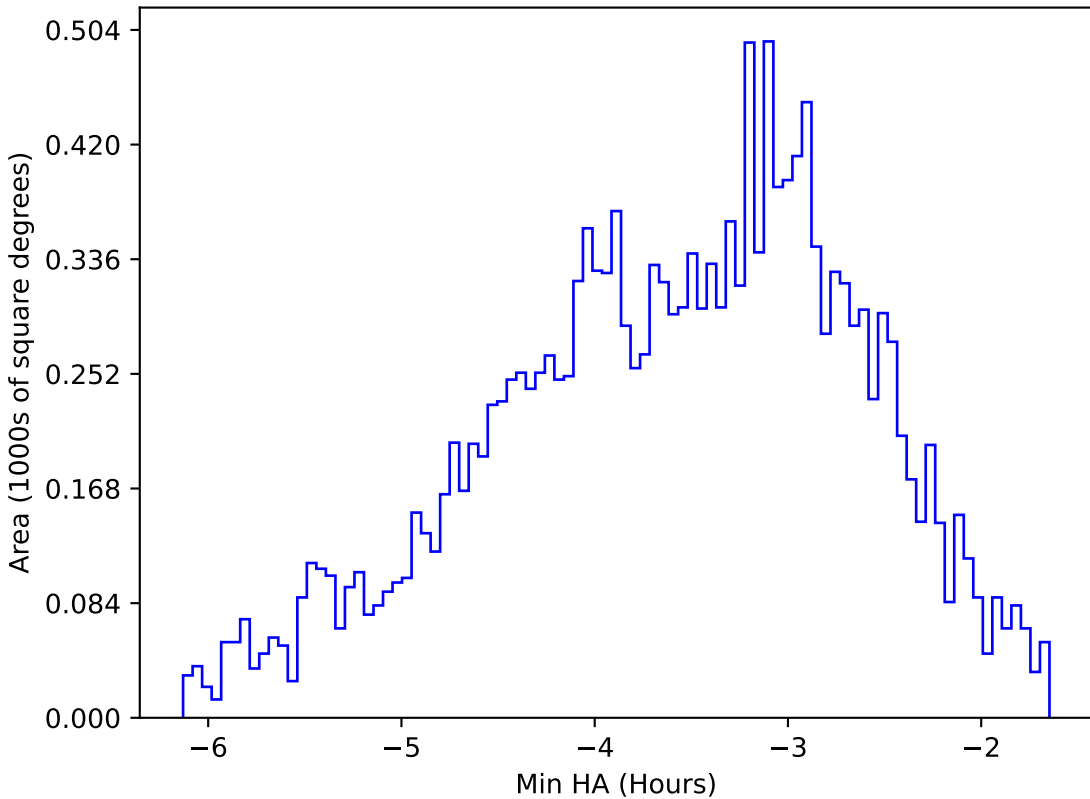
too_elab_r64_d3_giz_v3.4_10yrs WFD y band: Min HA
