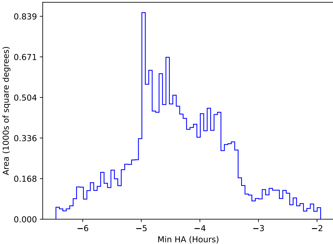
too_elab_r64_d3_giz_v3.4_10yrs WFD g band: Min HA
